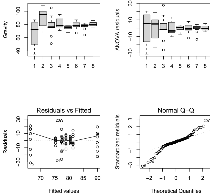
FIG 1. Gravity data and residual plots in Example 1 (sample sizes 8, 11, 9, 8, 8, 11, 13, and 13).
