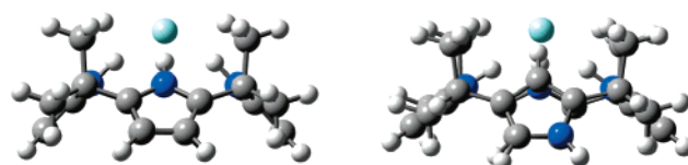
Figure 10. Calculated structures of 1 ·TMAF (calix[4]pyrrole·tetramethylammonium fluoride) and 2 ·TMAF complexes with 1:1 binding mode. Gaussian 03 64 was used for all calculations presented. For geometry optimizations the first guesses were fully optimized by PM3 semiempirical Hamiltonian. Then, the models were reoptimized at the B3LYP/6-31G* level of theory. The TMA + is omitted here for clarity (for more details see Supporting Information).
