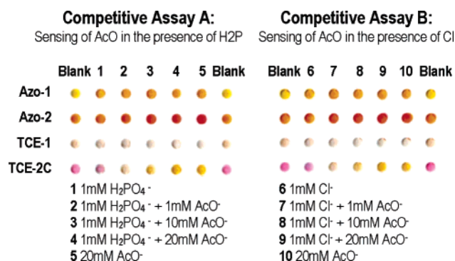
Figure 14. Competitive microarray utilizing Azo-1, Azo-2, TCE-1, and TCE-2C doped polyurethane. Assay A: Sensing of acetate (0–20 mM) administered as an aqueous solution containing 1 mM \text{H}_2\text{PO}_4^- . Assay B: Sensing of acetate (0–20 mM) administered as an aqueous solution containing 1 mM \text{Cl}^- .
