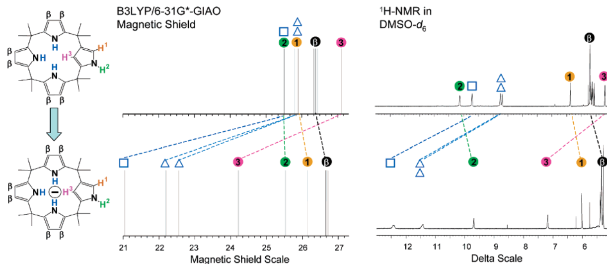
Figure 11. (a) Calculated DFT-GIAO magnetic shields for NC-OMCP and NC-OMCP·TMAF in 1:1 binding mode at the B3LYP/6-31G* level of theory. (b) 1 H-NMR of 2 ( 1.0 \times 10^{-2} M) in DMSO- d 6 before and after the addition of 1.85 equiv of TBAF. For details see Supporting Information.
